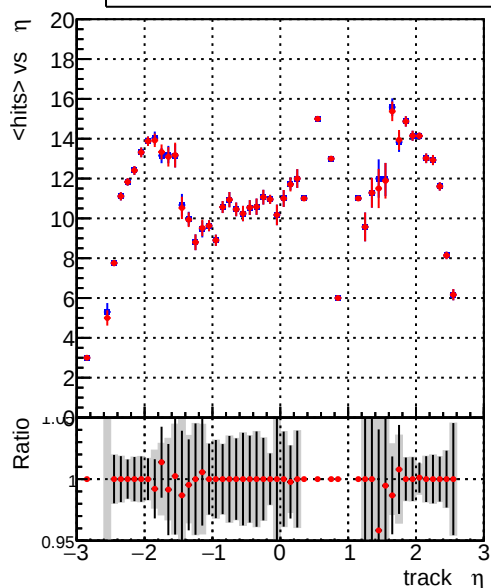
Baseline_TTBarPU_600events_2025_CATunedParams mean hits vs \eta PR_TTBarPU_600events_2025_CATunedParams
