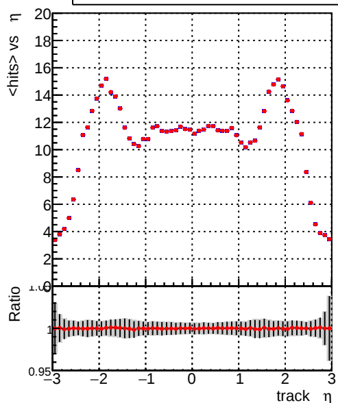
mean hits vs \eta Baseline_TTBarPU_600events_2025_CATunedParams PR_TTBarPU_600events_2025_CATunedParams
